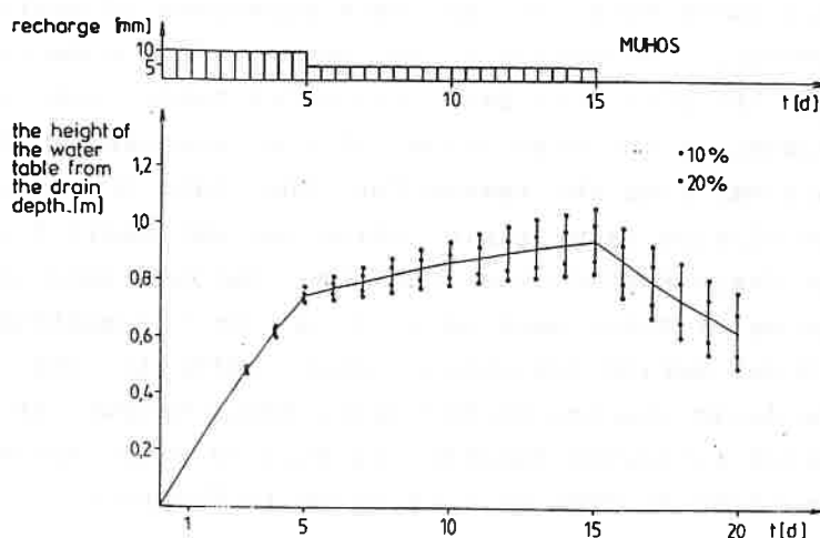
Fig. 6. The effects of a 10% and 20% variation in the value of the hydraulic conductivity on water table height in the sandy loam field.
